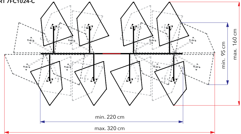
8 FLAP CHANDELIER PART 7FC1024-C
