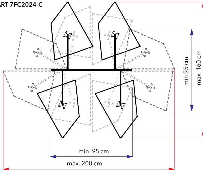
4 FLAP CHANDELIER PART 7FC2024-C
